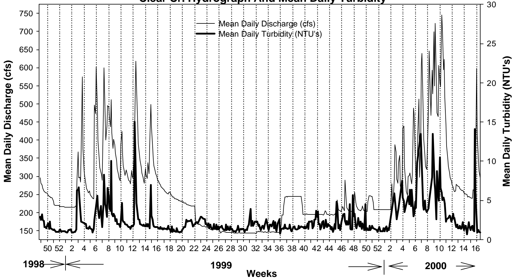
Figure 4. Mean daily discharge (cfs) and turbidity (NTU's) for Clear Cr. (SM 1.7) for the period 5 December 1998 through 21 April 2000.
