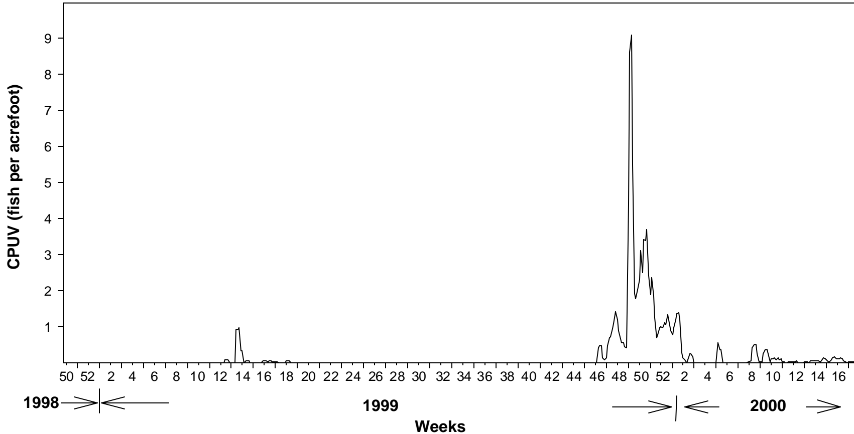
Figure 12. Summary of catch per unit volume (CPUV) expressed in fish per acrefoot for spring chinook salmon captured by rotary-screw trap on Clear Creek (stream mile 1.7). Run designation was assigned based on length criteria developed by the California Department of Water Resources. Each data point represents a three day rolling average of CPUV comprised of the day before, the day of, and the day after the sample was gathered.
