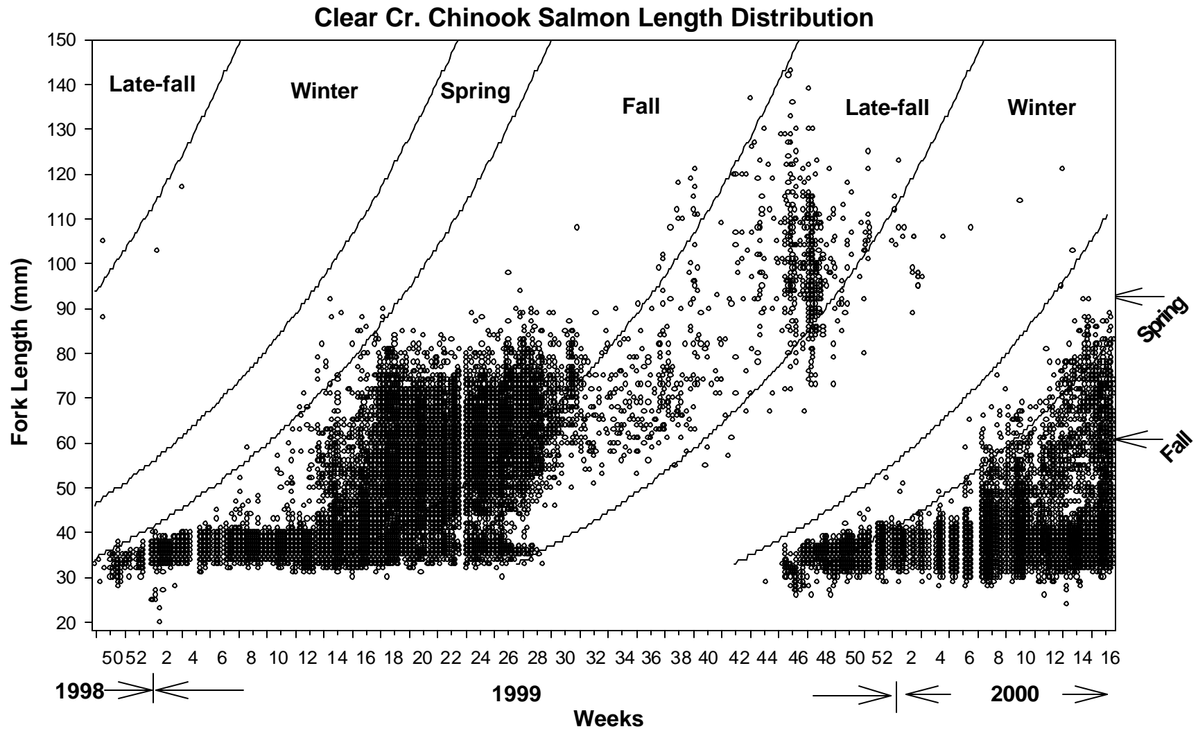
Figure 7. Daily fork length distribution by run for Chinook salmon captured by rotary-screw trap on Clear Cr. (SM1.7) for the period 5 December 1998 through 21 April 2000. Spline curves represent the maximum fork length expected by date for each run, based on criteria developed by the California Department of Water Resources.
