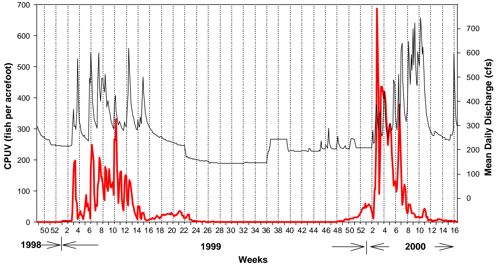
Figure 6. Summary of catch per unit volume (CPUV) expressed in fish per acrefoot for fall chinook salmon captured by rotary-screw trap on Clear Creek (stream mile 1.7) for the period 5 December through 21 April. Run designation was assigned based on length criteria developed by the California Department of Water Resources. Each data point represents a three day rolling average of CPUV comprised of the day before, the day of, and the day after the sample was gathered. Mean daily flow is presented as discharge (cfs).
