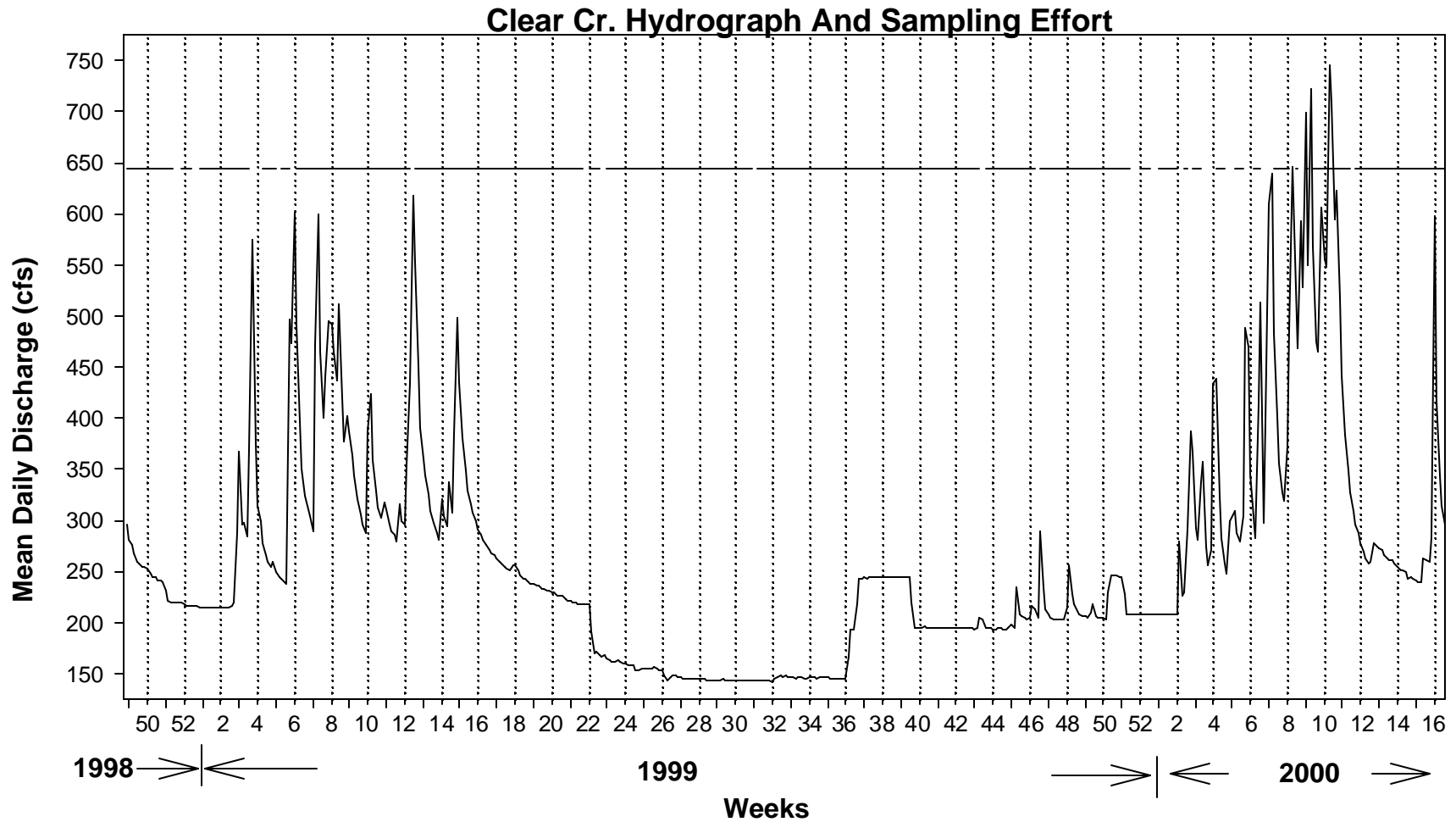
Figure 2. Daily mean discharge (cfs) and rotary-trapping effort on Clear Cr. (SM 1.7) from 5 December 1998 through 21 April 2000. The horizontal dashed line indicates 24-hr. samples. Breaks in the line represent days when rotary trapping was not conducted (usually due to high flow events).
