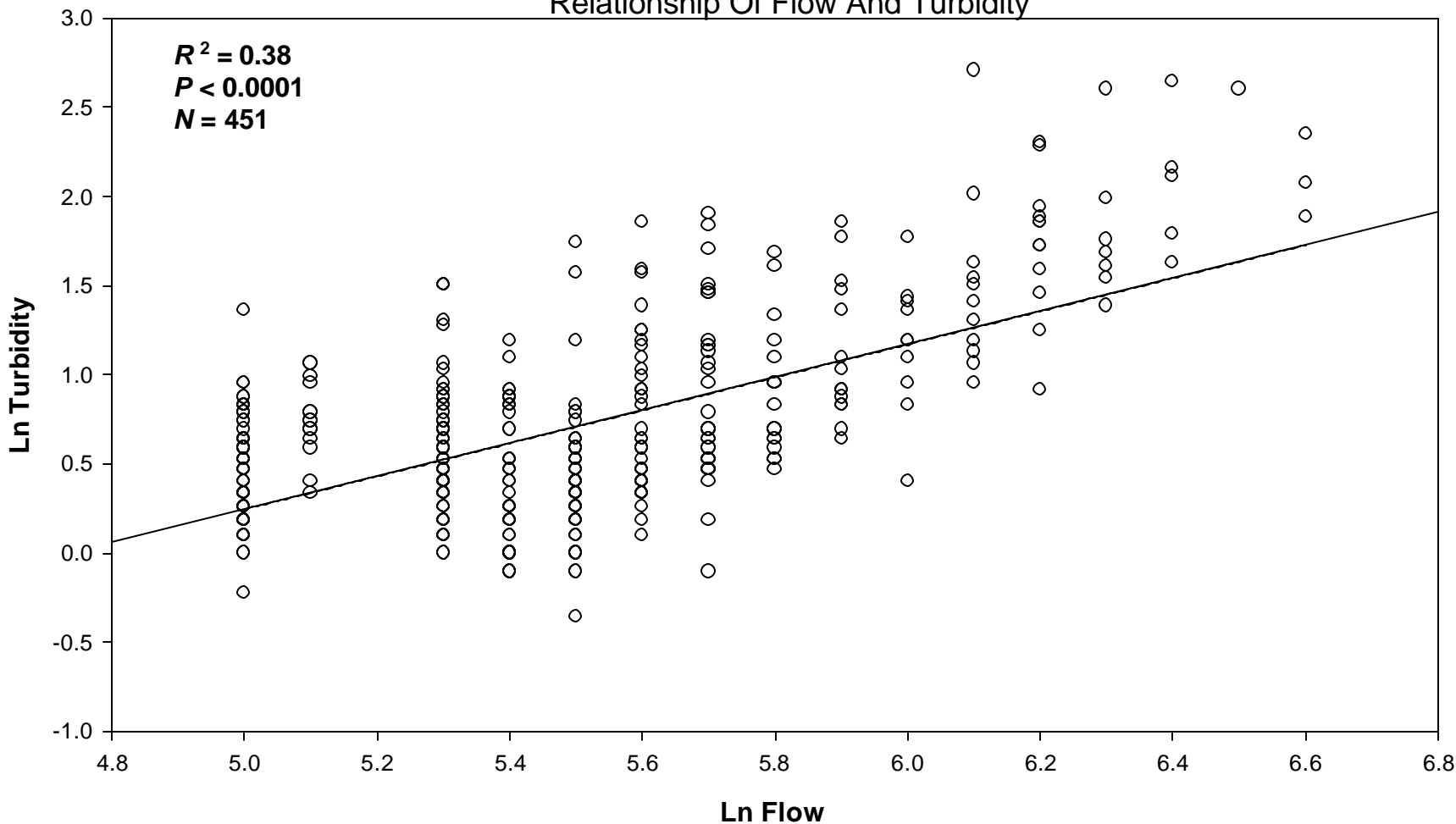
Figure 5. Relationship of flow and turbidity for Clear Creek (SM 1.7) from 5 December 1998 through 21 April 2000. Raw data was log transformed (Ln) to standardize error variance. A least squares regression line was then fitted to the data to explain the relationship of these two variables. Flow was a moderate predictor of turbidity with R^2 = 0.38 and the slope of the least squares regression line was significantly different than zero.
