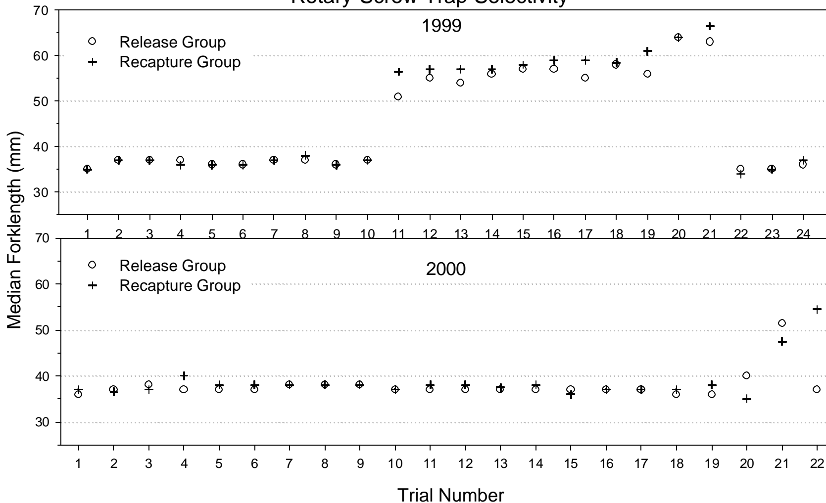
Figure 16. Summary of mark/recapture trials evaluating rotary-screw trap selectivity. Data represent the median fork length (mm) of marked and recaptured chinook salmon on Clear Cr. (SM 1.7) for the period 5 December 1998 through 21 April 2000. Note that no trials were conducted in December of 1998.
