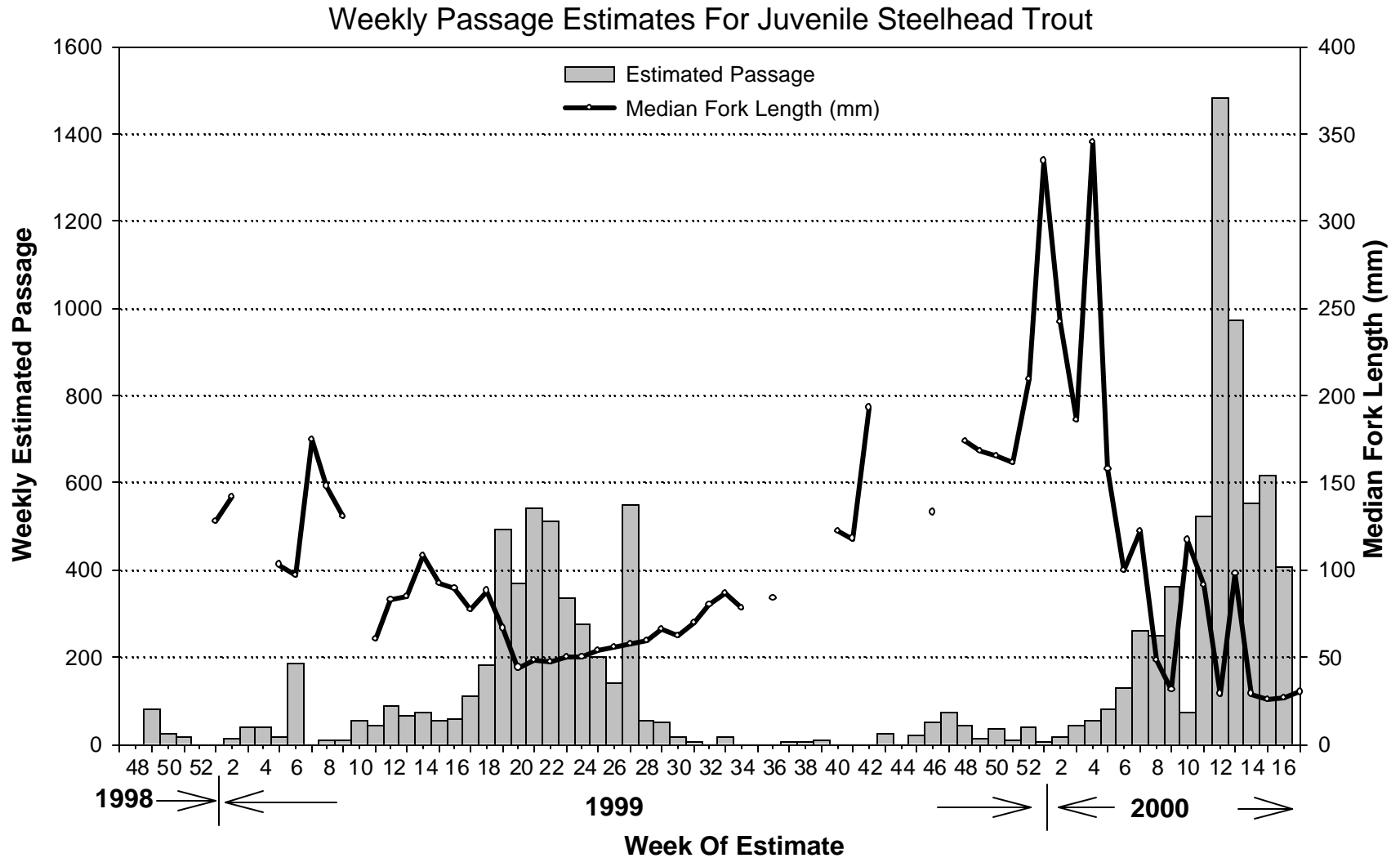
Figure 21. Weekly estimated passage of juvenile steelhead trout from Clear Creek (SM 1.7) for the period 5 December 1998 through 21 April 2000. Estimates were derived by summing the total catch for a given week and dividing that number by trap efficiency. Trap efficiencies were generated through the use of multiple mark/recapture trials.
